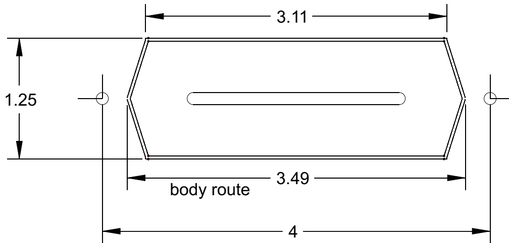
CC ARCHTOP 2 POINT MOUNTING
